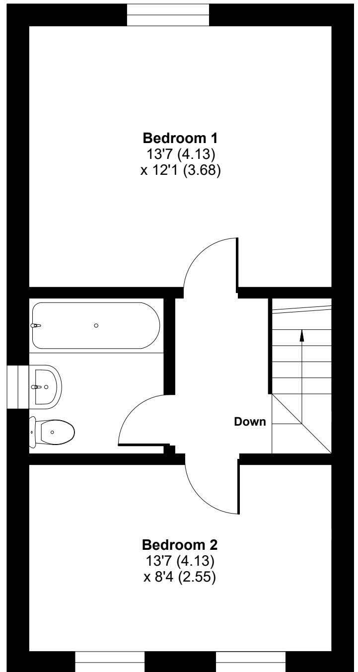
FIRST FLOOR
